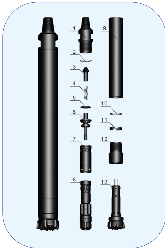
HR-4D DTH Hammers
